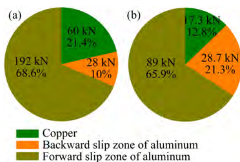
Fig. 10 Rolling force ratios of copper strip and aluminum cladding when T_{\text{Casting}}=700 °C: (a) H_{Cu}=0.5 mm, V=2.4 m/min; (b) H_{Cu}=0.5 mm, V=3.6 m/min
