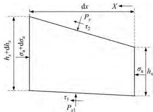
Fig. 4 Stress analysis of micro unit in substrate strip
